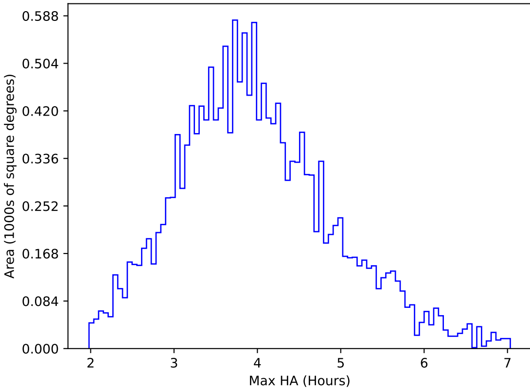
too_elab_r8_d3_griz_v3.4_10yrs WFD u band: Max HA
