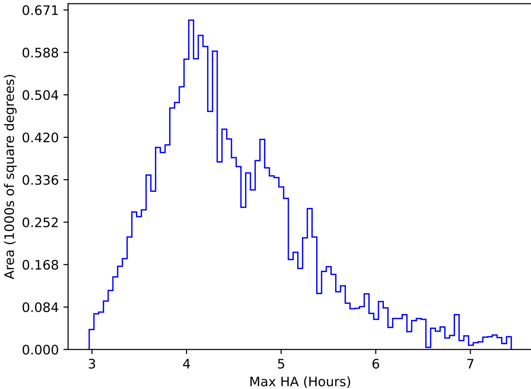
too_elab_r8_d3_griz_v3.4_10yrs WFD r band: Max HA
