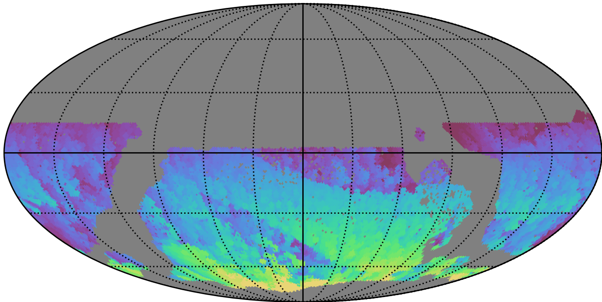
too_elab_r8_d3_griz_v3.4_10yrs WFD i band: Max HA
