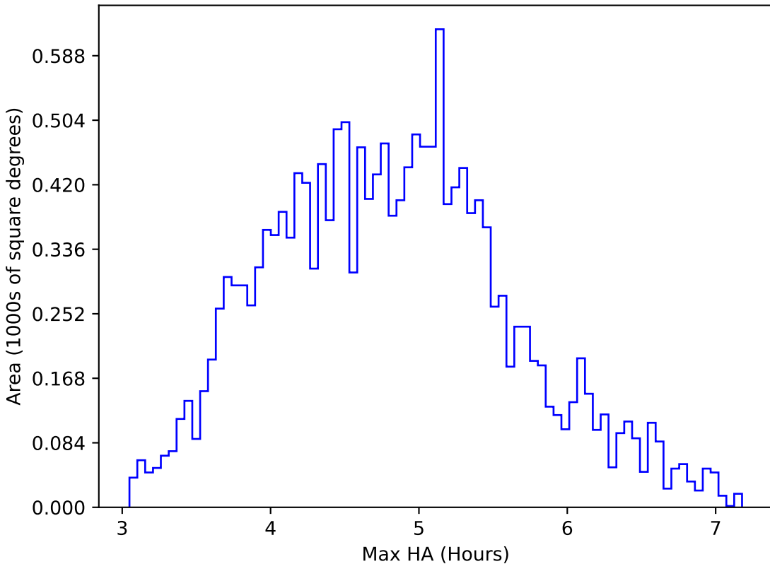
too_elab_r8_d3_griz_v3.4_10yrs WFD i band: Max HA
