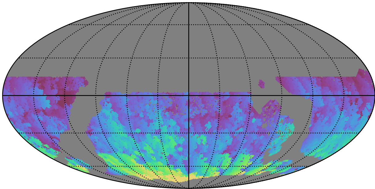
too_elab_r8_d3_griz_v3.4_10yrs WFD g band: Max HA
