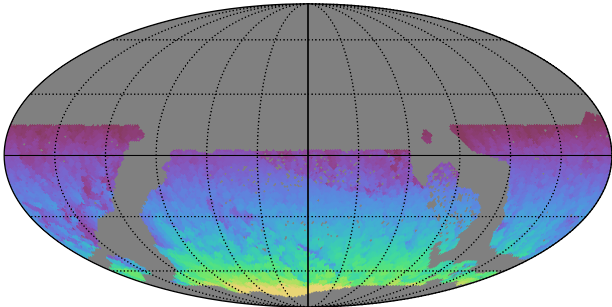
too_elab_r8_d3_griz_v3.4_10yrs WFD all bands: Max HA
