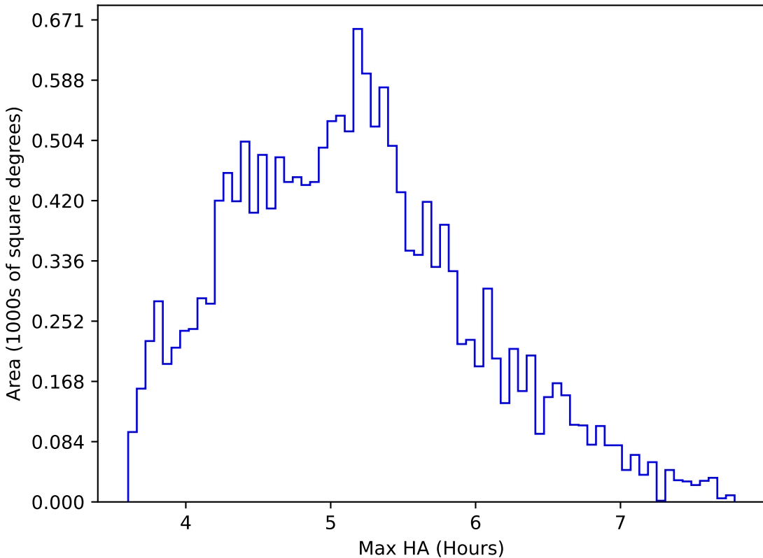
too_elab_r8_d3_griz_v3.4_10yrs WFD all bands: Max HA
