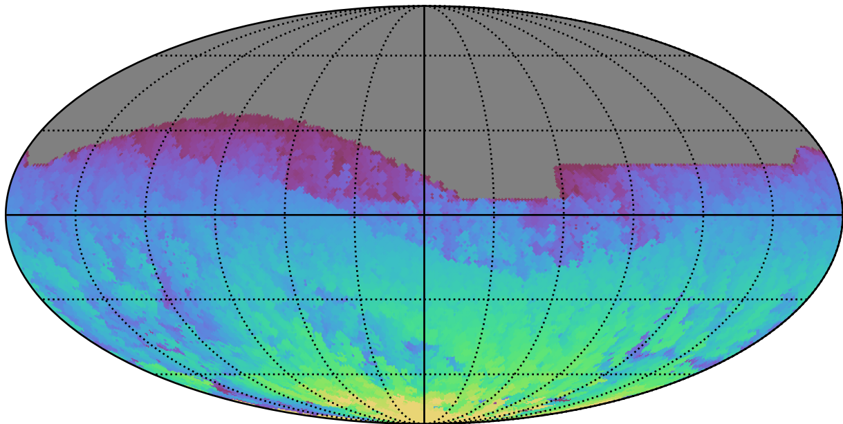
too_elab_r8_d3_griz_v3.4_10yrs All sky z band: Max HA
