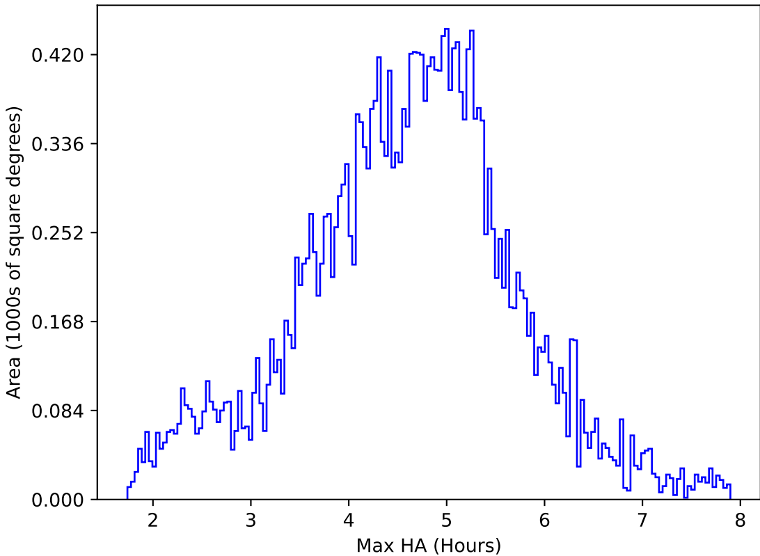
too_elab_r8_d3_griz_v3.4_10yrs All sky z band: Max HA
