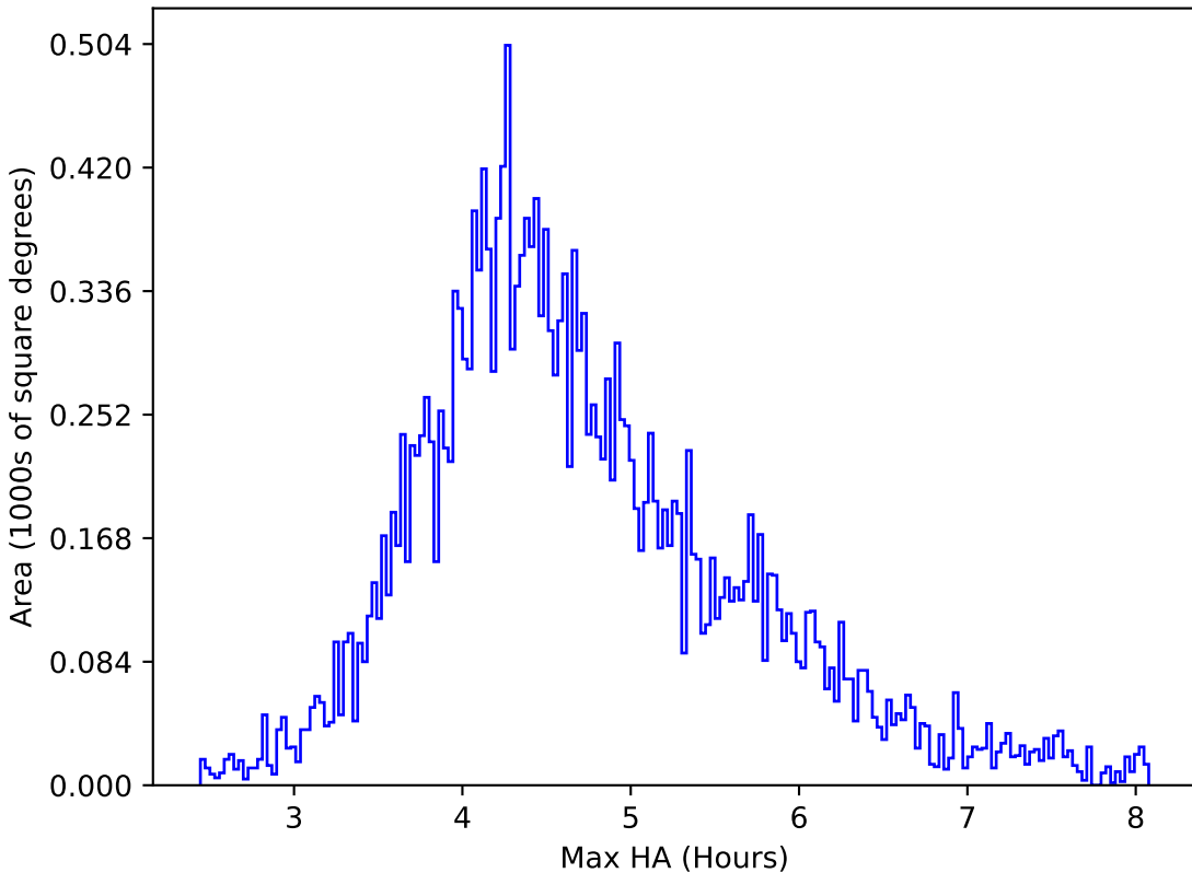
too_elab_r8_d3_griz_v3.4_10yrs All sky y band: Max HA
