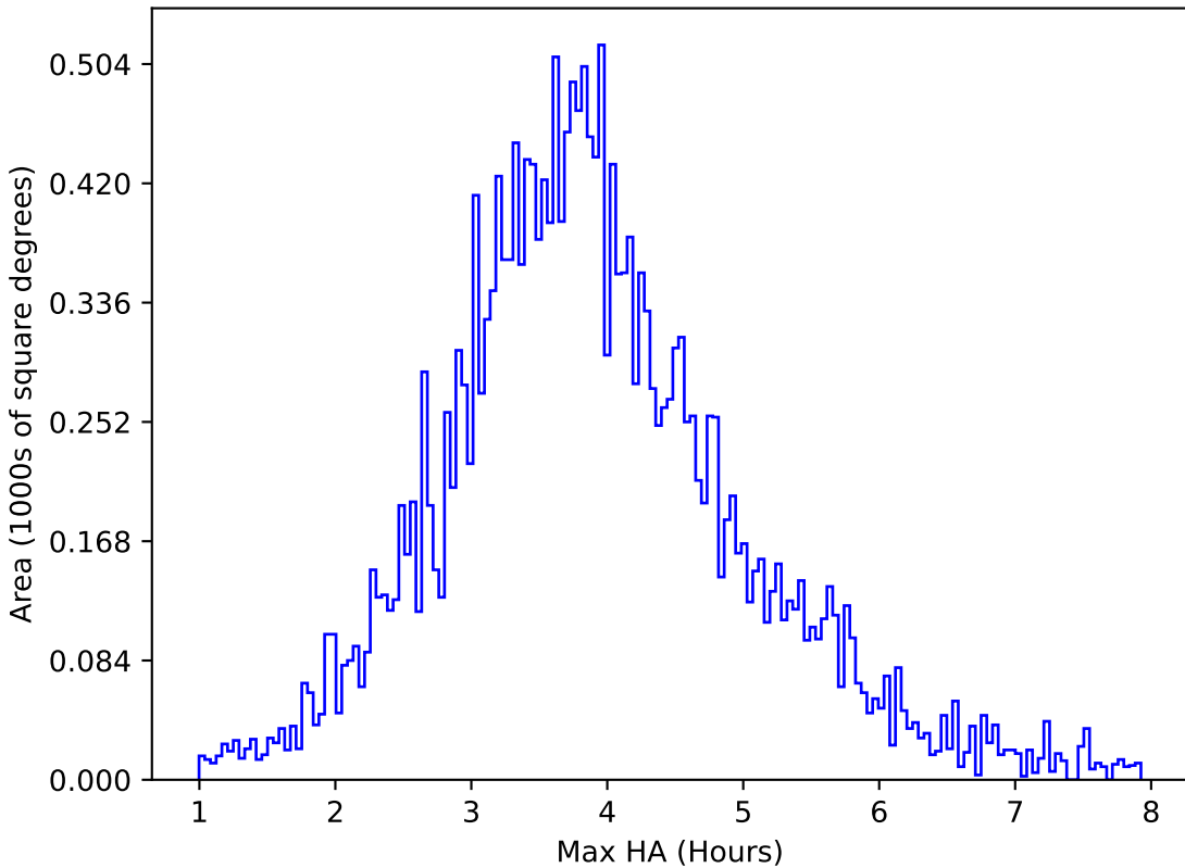
too_elab_r8_d3_griz_v3.4_10yrs All sky u band: Max HA
