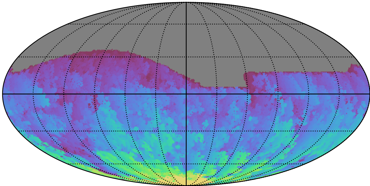
too_elab_r8_d3_griz_v3.4_10yrs All sky g band: Max HA
