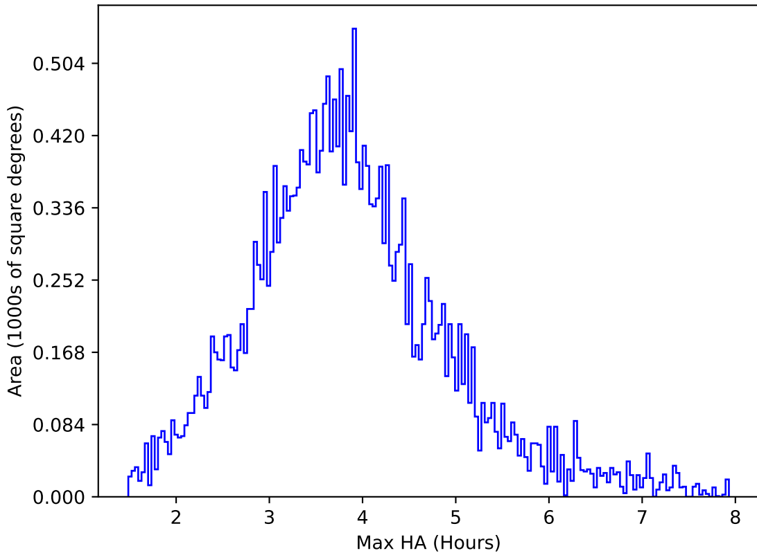
too_elab_r8_d3_griz_v3.4_10yrs All sky g band: Max HA
