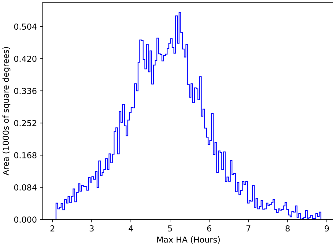
too_elab_r8_d3_griz_v3.4_10yrs All sky all bands: Max HA
