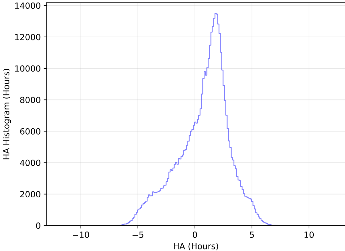
too_elab_r8_d3_griz_v3.4_10yrs WFD z band: HA Histogram
