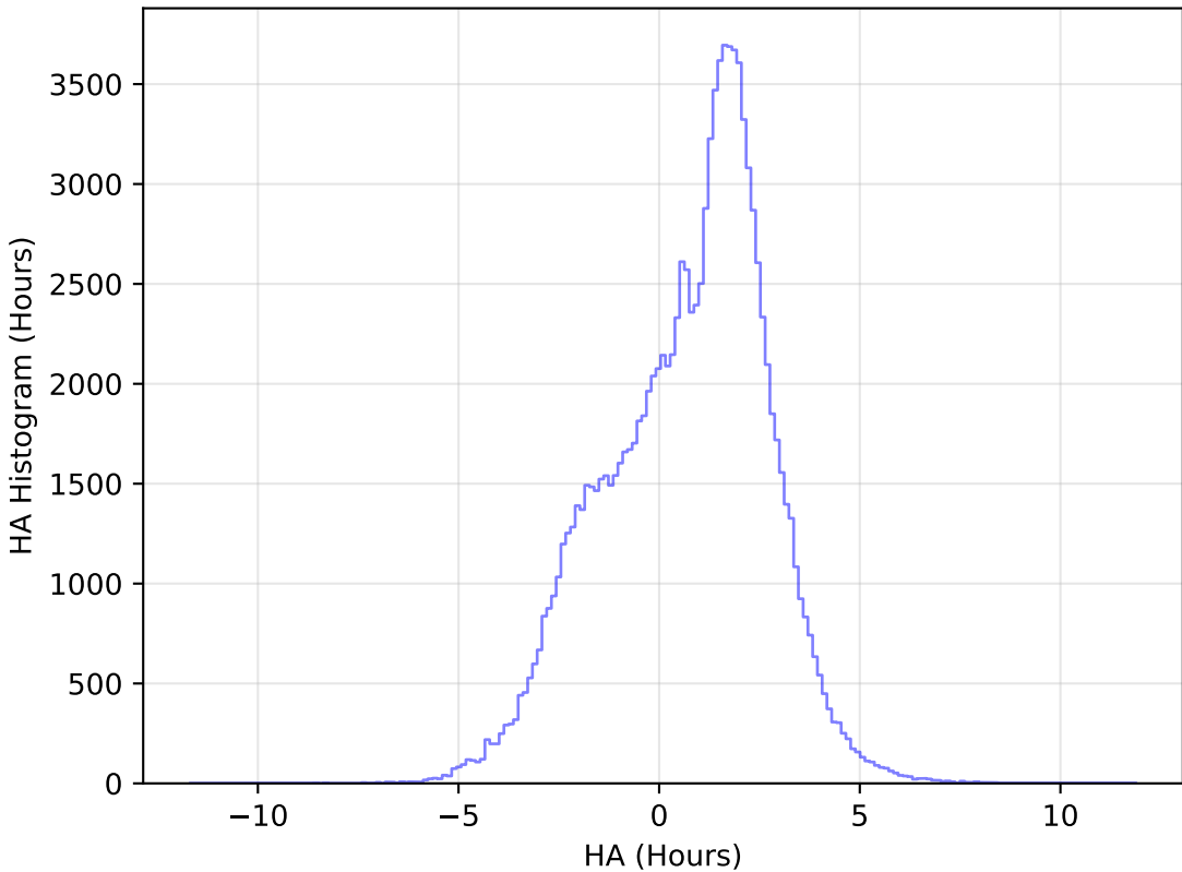
too_elab_r8_d3_griz_v3.4_10yrs WFD u band: HA Histogram
