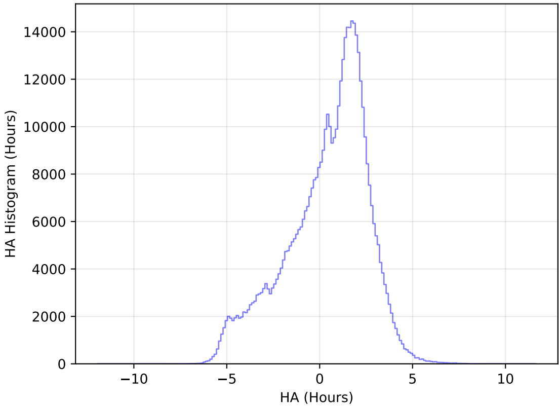
too_elab_r8_d3_griz_v3.4_10yrs WFD r band: HA Histogram
