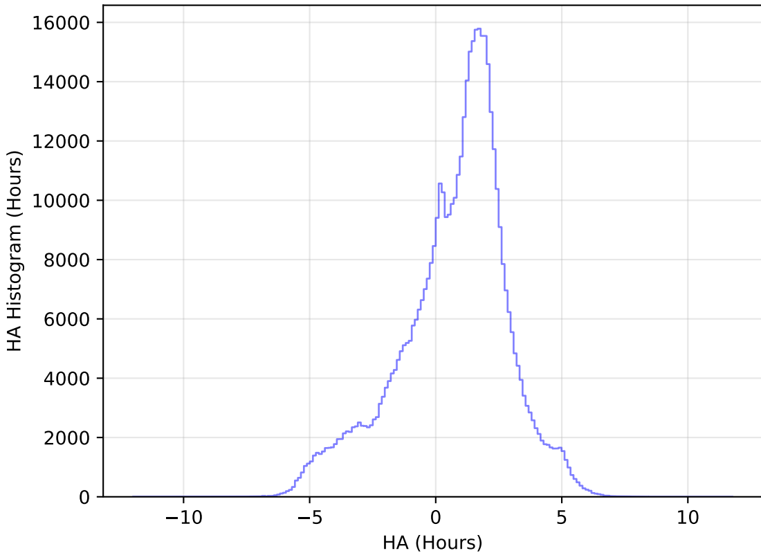
too_elab_r8_d3_griz_v3.4_10yrs WFD i band: HA Histogram
