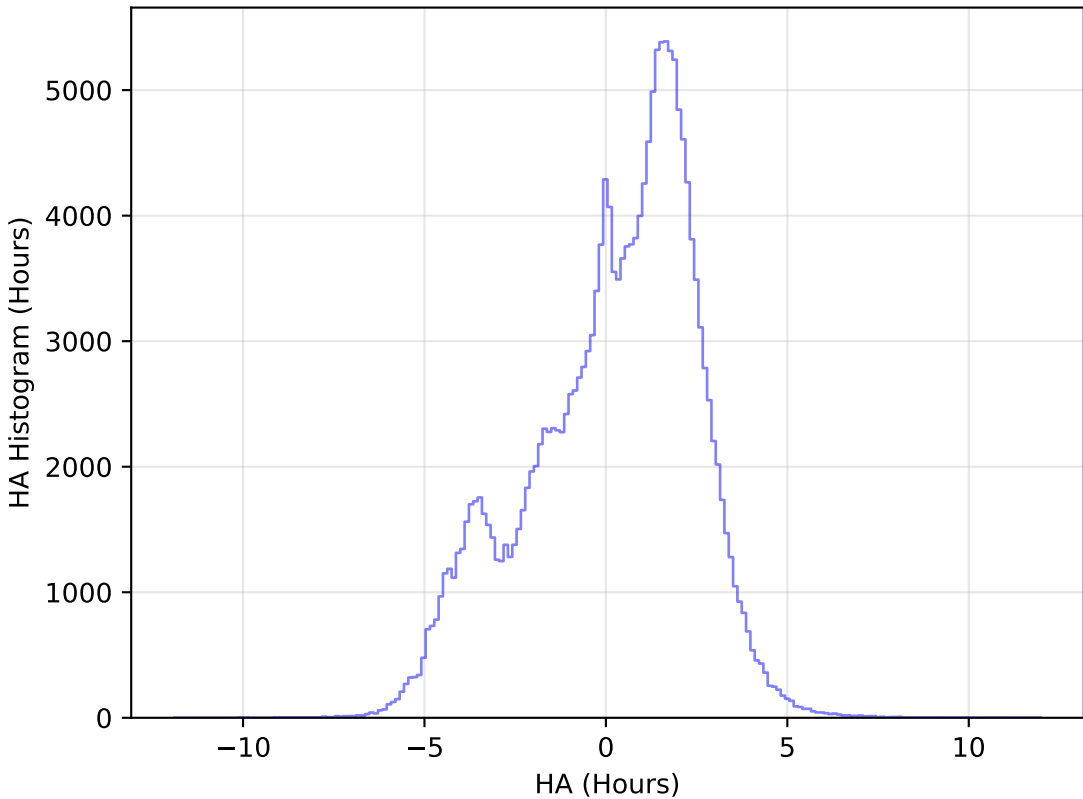
too_elab_r8_d3_griz_v3.4_10yrs WFD g band: HA Histogram
