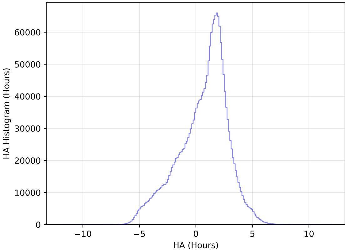
too_elab_r8_d3_griz_v3.4_10yrs WFD all bands: HA Histogram
