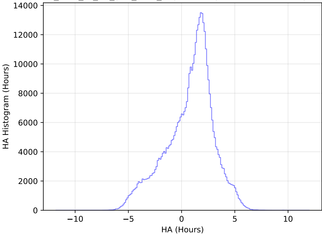
too_elab_r8_d3_griz_v3.4_10yrs All sky z band: HA Histogram
