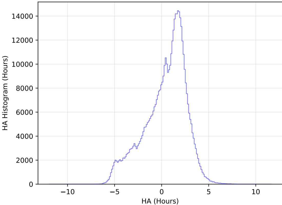
too_elab_r8_d3_griz_v3.4_10yrs All sky r band: HA Histogram
