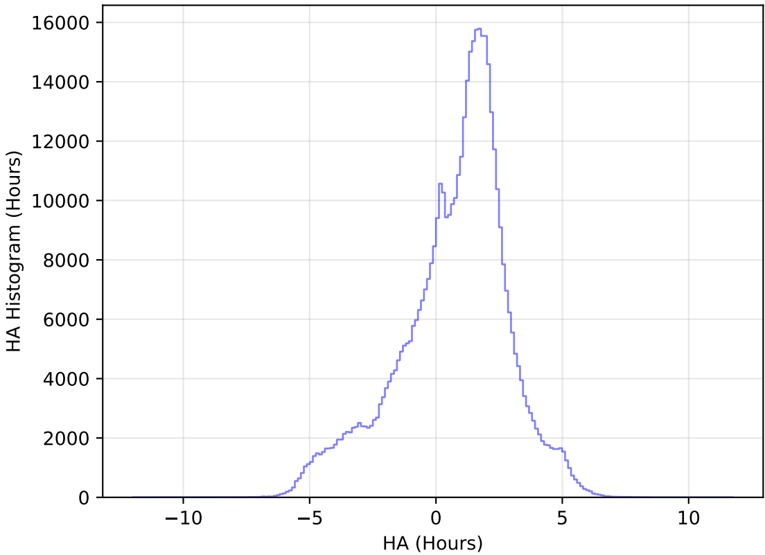
too_elab_r8_d3_griz_v3.4_10yrs All sky i band: HA Histogram
