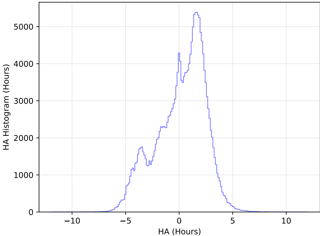
too_elab_r8_d3_griz_v3.4_10yrs All sky g band: HA Histogram
