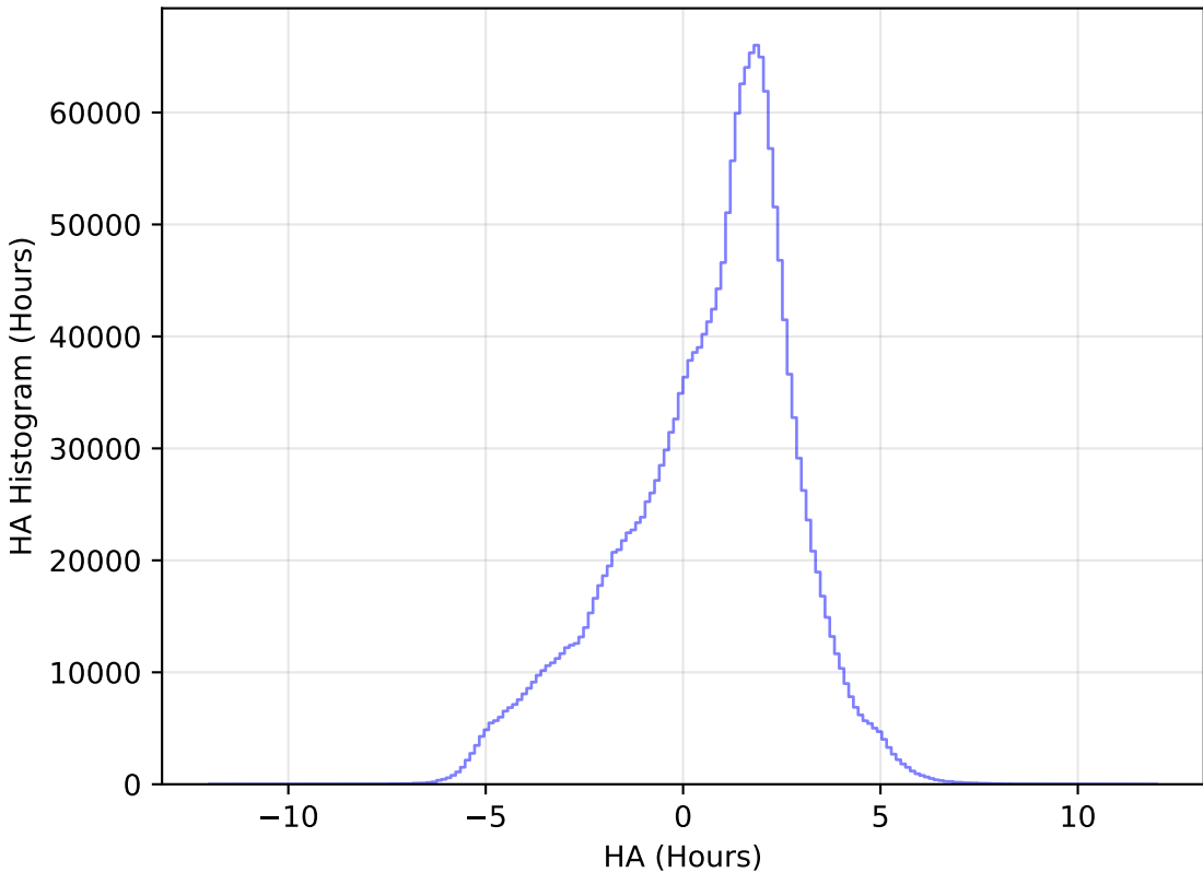
too_elab_r8_d3_griz_v3.4_10yrs All sky all bands: HA Histogram
