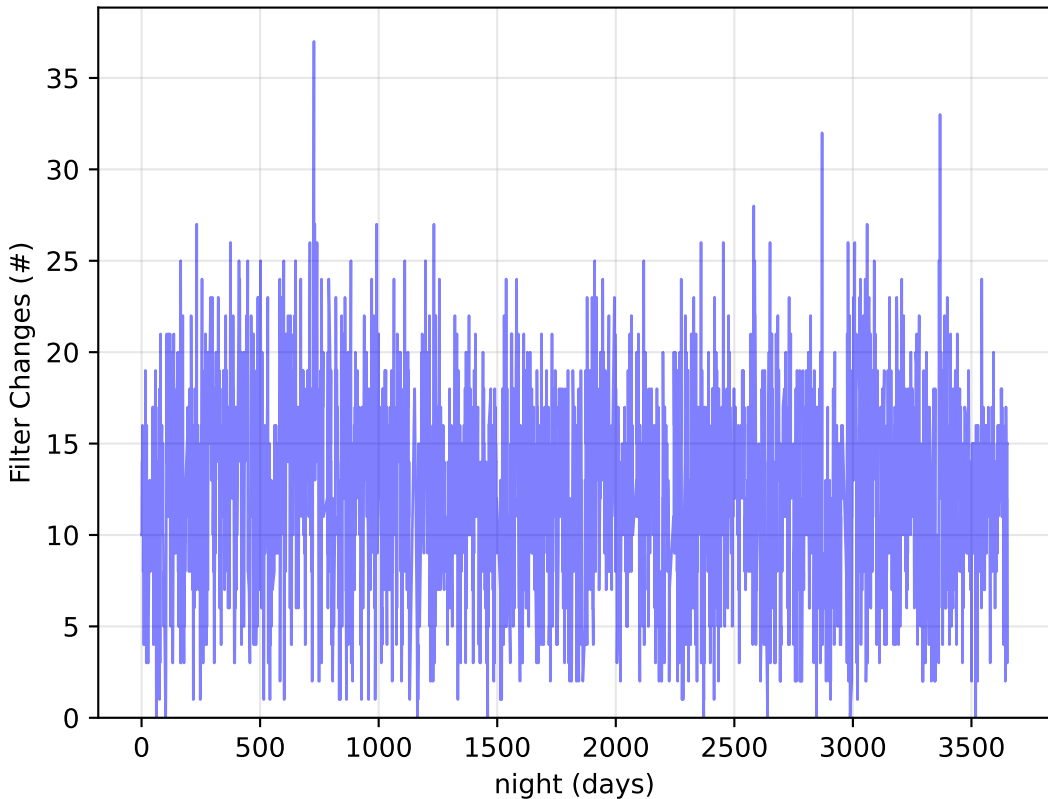
too_elab_r8_d3_griz_v3.4_10yrs Per Night: Filter Changes
