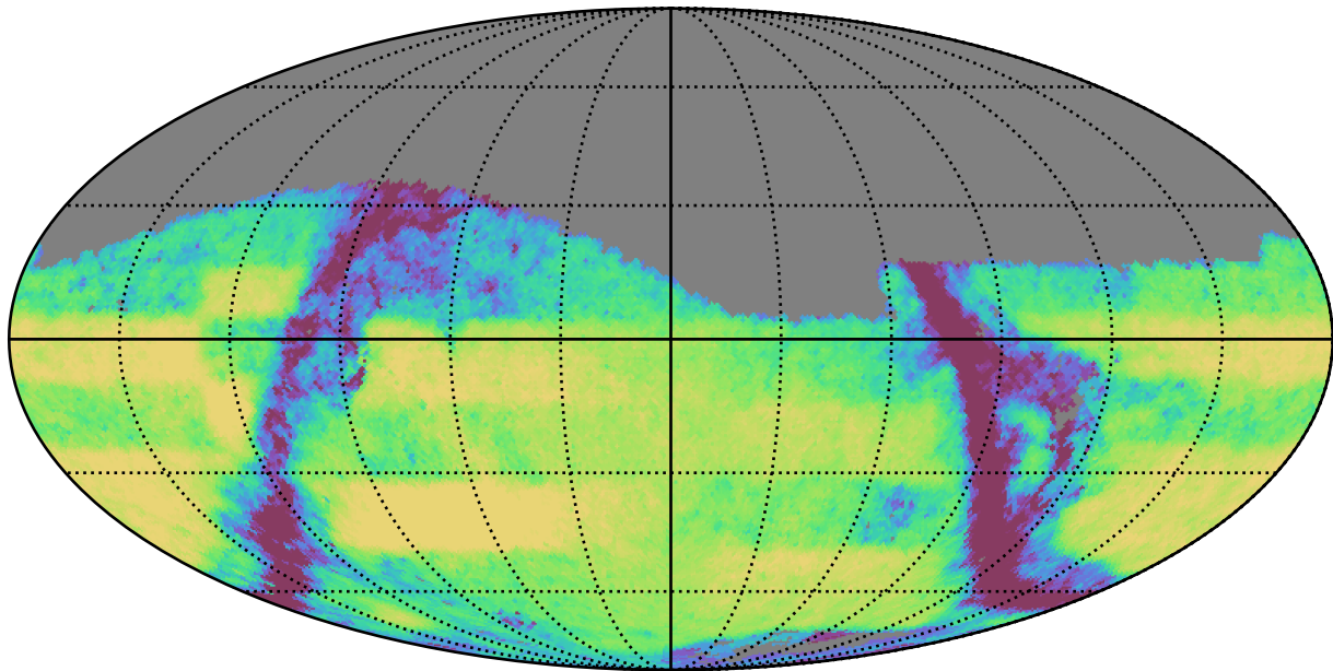
too_elab_r8_d3_griz_v3.4_10yrs Yr 3-4 r band: Exgal_CoaddM5
