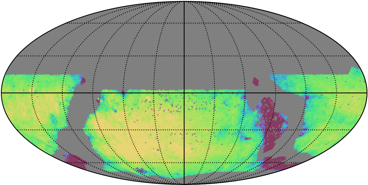
too_elab_r8_d3_griz_v3.4_10yrs WFD g band: Exgal_CoaddM5
