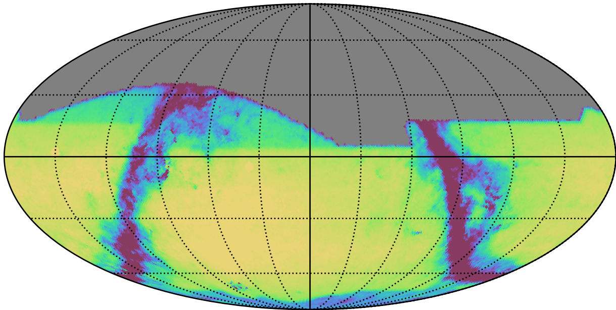
too_elab_r8_d3_griz_v3.4_10yrs All sky r band: Exgal_CoaddM5
