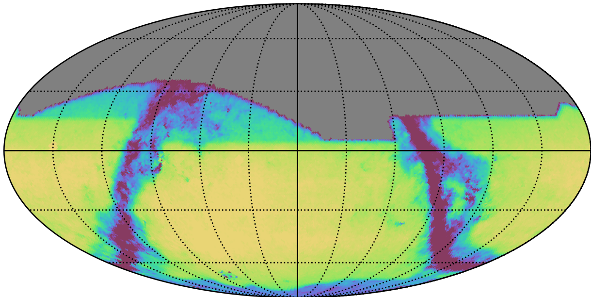
too_elab_r8_d3_griz_v3.4_10yrs All sky i band: Exgal_CoaddM5
