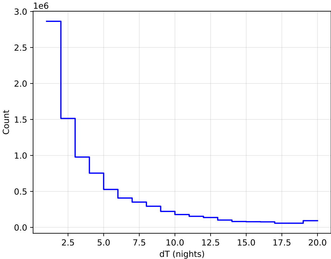
too_elab_r8_d3_griz_v3.4_10yrs All sky all bands: DeltaNight Histogram
