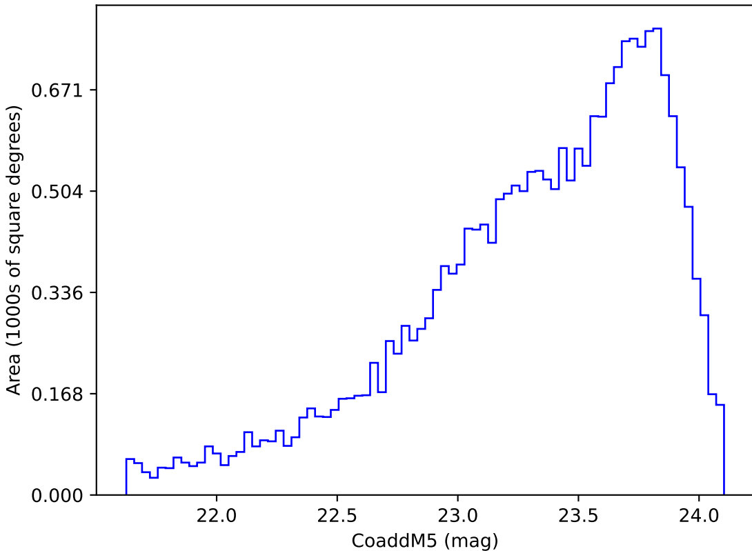
too_elab_r8_d3_griz_v3.4_10yrs Yr 3-4 y band: CoaddM5
