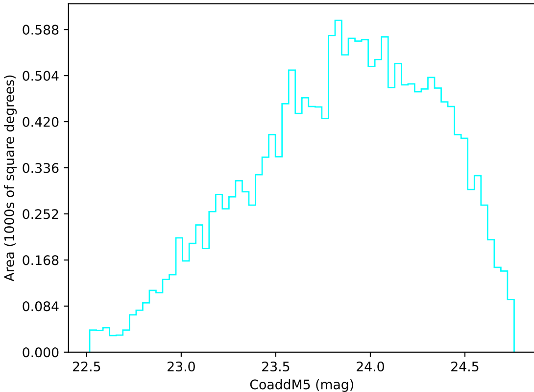
too_elab_r8_d3_griz_v3.4_10yrs Yr 3-4 u band: CoaddM5
