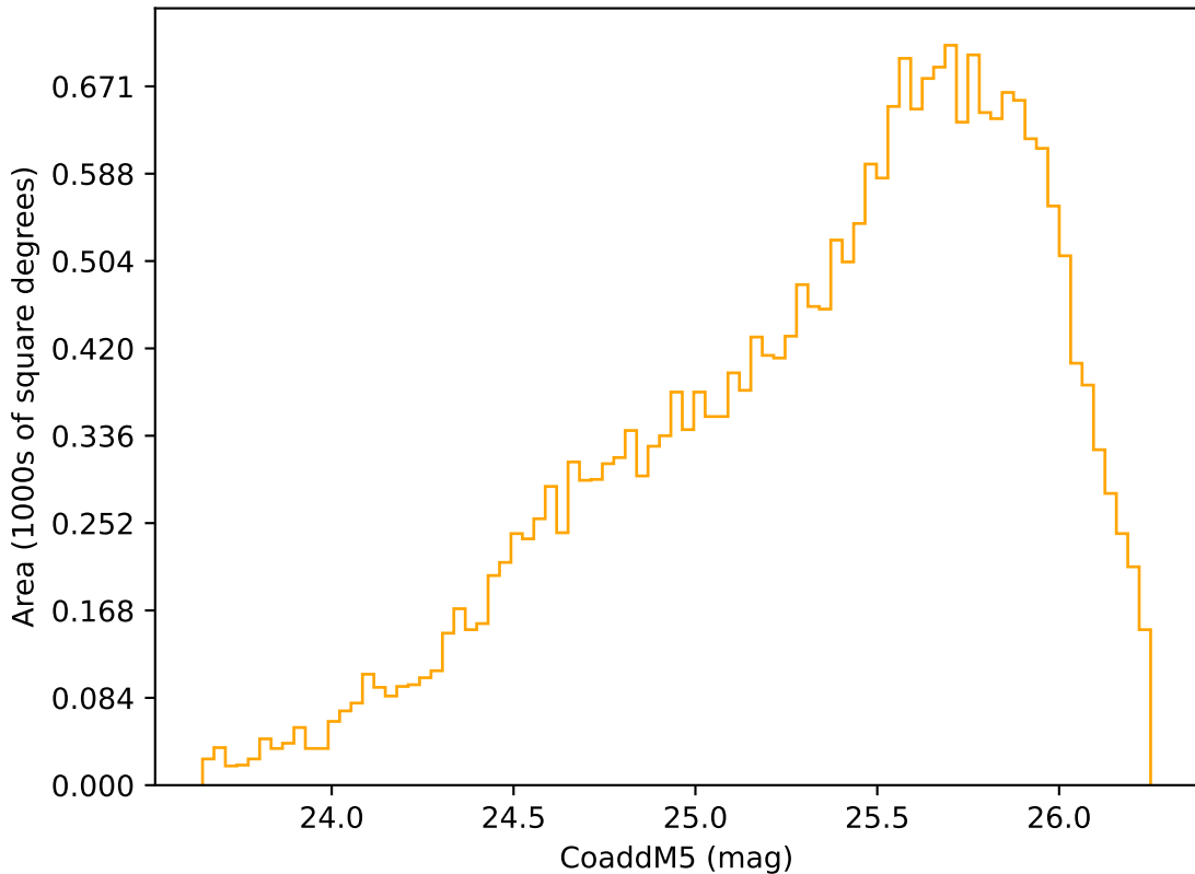
too_elab_r8_d3_griz_v3.4_10yrs Yr 3-4 r band: CoaddM5
