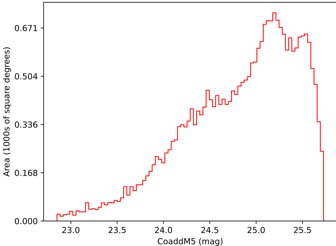
too_elab_r8_d3_griz_v3.4_10yrs Yr 3-4 i band: CoaddM5
