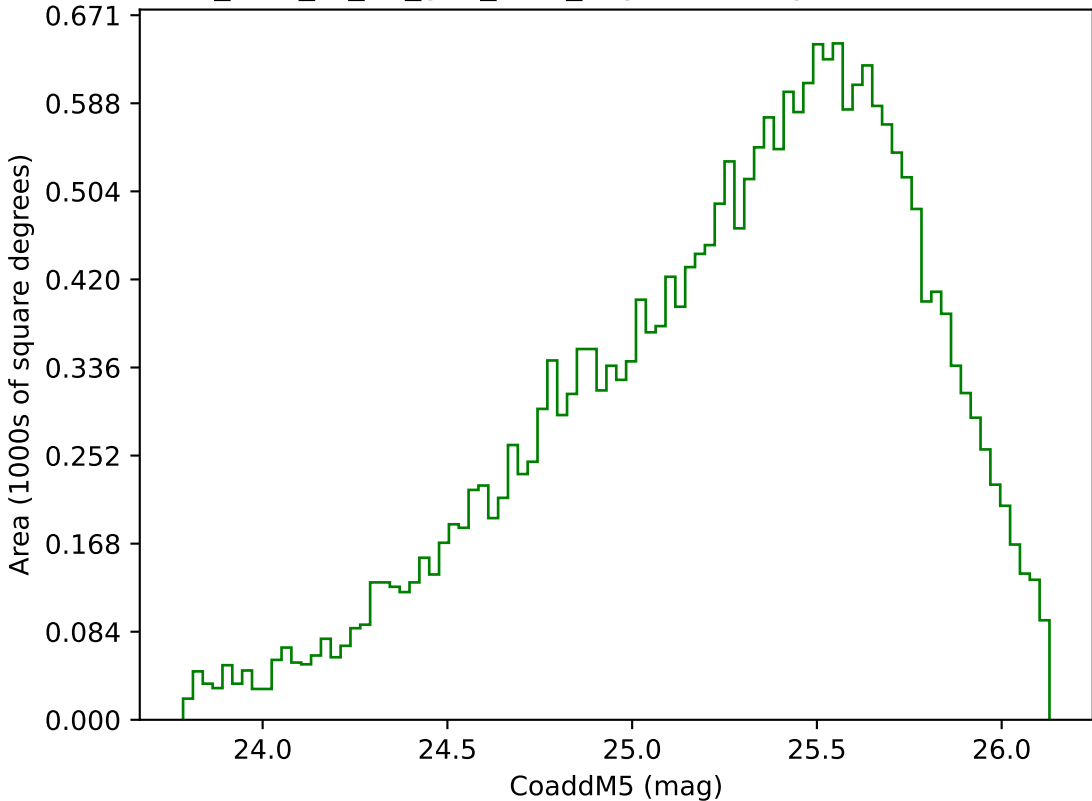
too_elab_r8_d3_griz_v3.4_10yrs Yr 3-4 g band: CoaddM5
