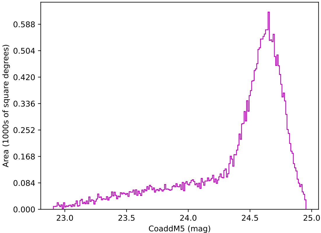
too_elab_r8_d3_griz_v3.4_10yrs Yr 1 z band: CoaddM5
