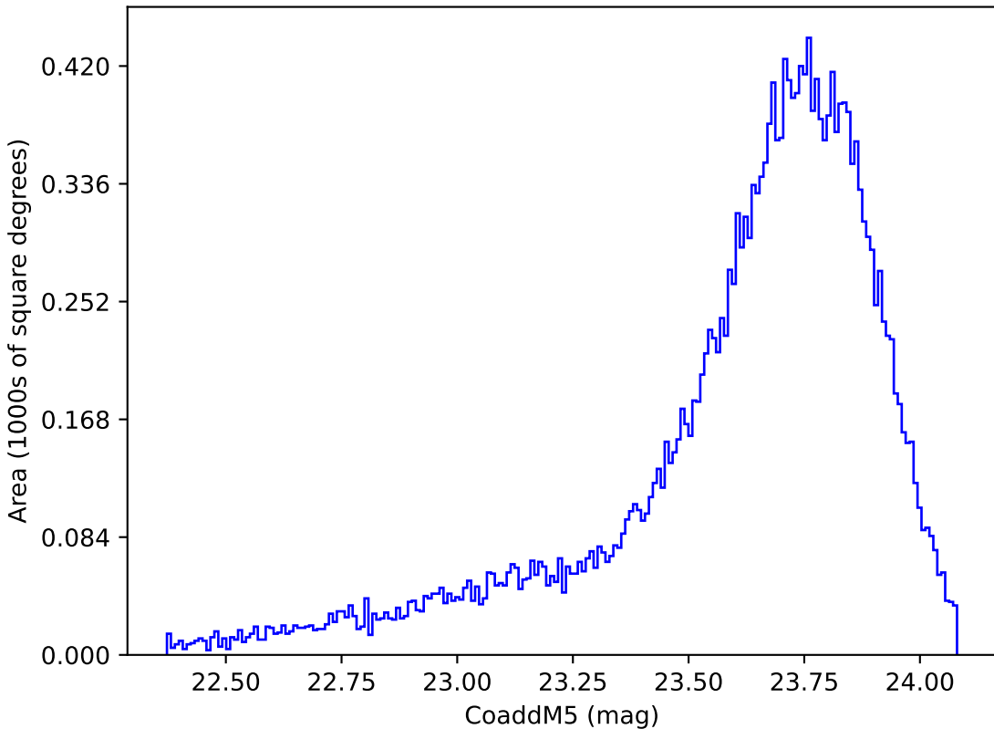
too_elab_r8_d3_griz_v3.4_10yrs Yr 1 y band: CoaddM5
