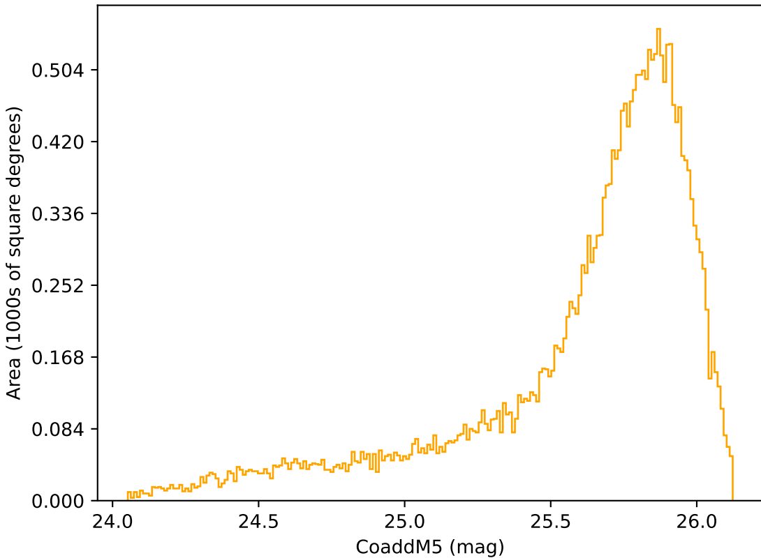
too_elab_r8_d3_griz_v3.4_10yrs Yr 1 r band: CoaddM5
