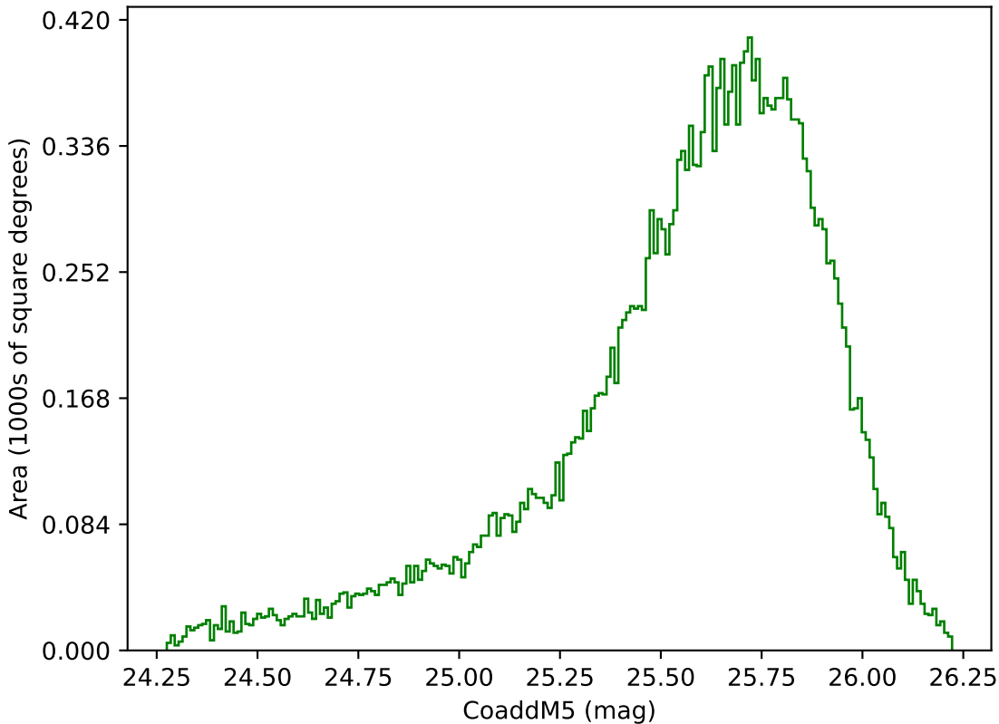
too_elab_r8_d3_griz_v3.4_10yrs Yr 1 g band: CoaddM5
