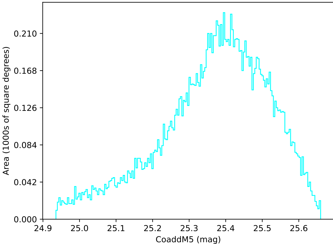
too_elab_r8_d3_griz_v3.4_10yrs WFD u band: CoaddM5
