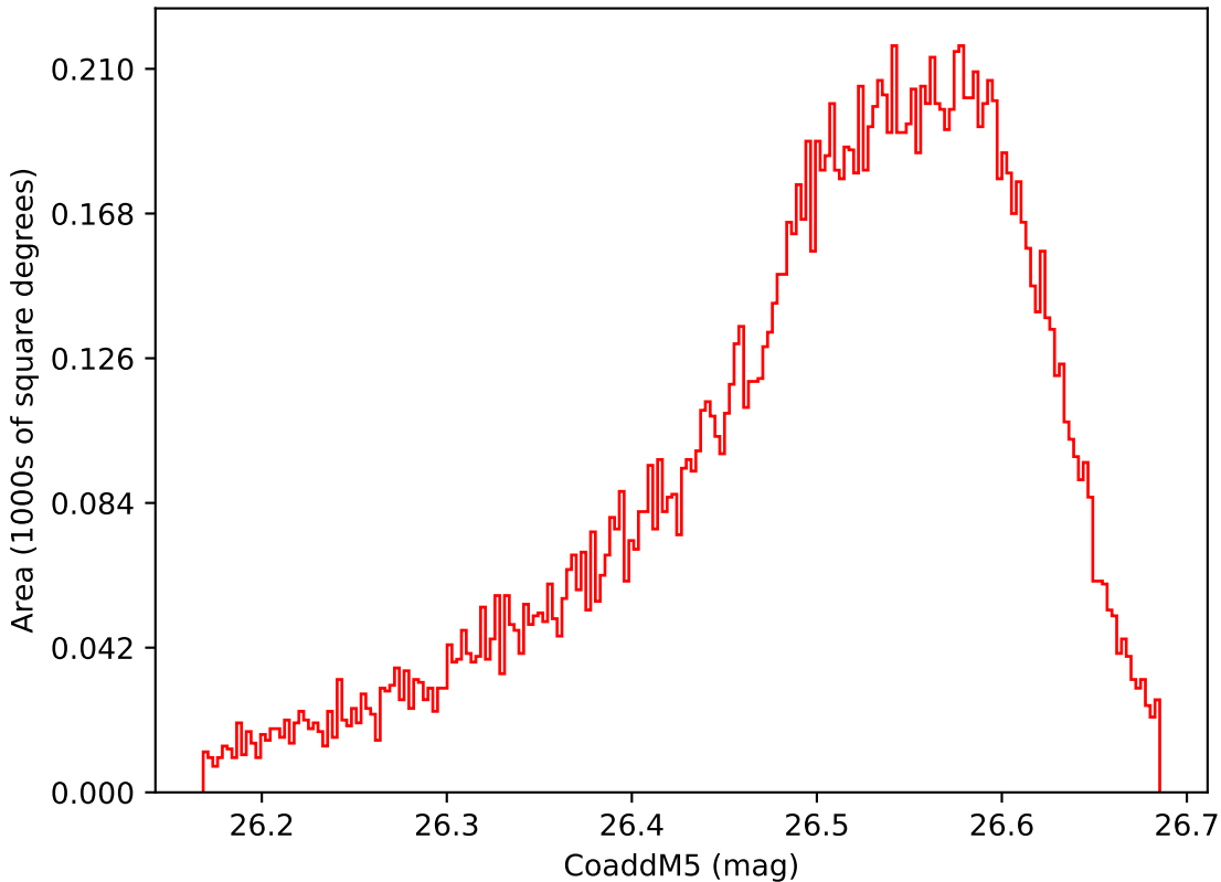
too_elab_r8_d3_griz_v3.4_10yrs WFD i band: CoaddM5
