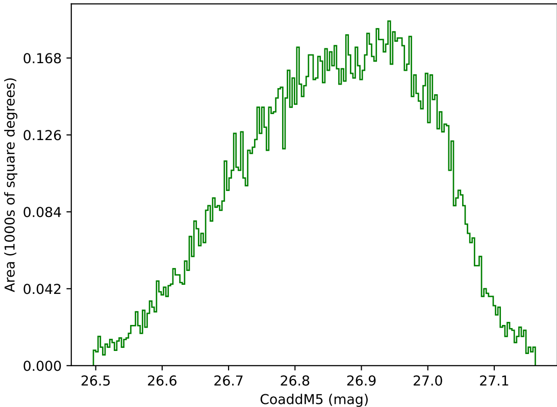
too_elab_r8_d3_griz_v3.4_10yrs WFD g band: CoaddM5
