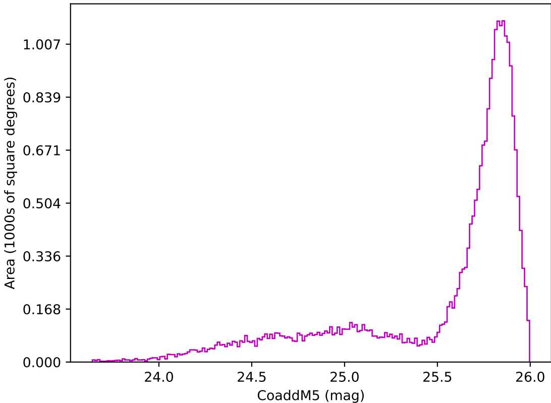
too_elab_r8_d3_griz_v3.4_10yrs All sky z band: CoaddM5
