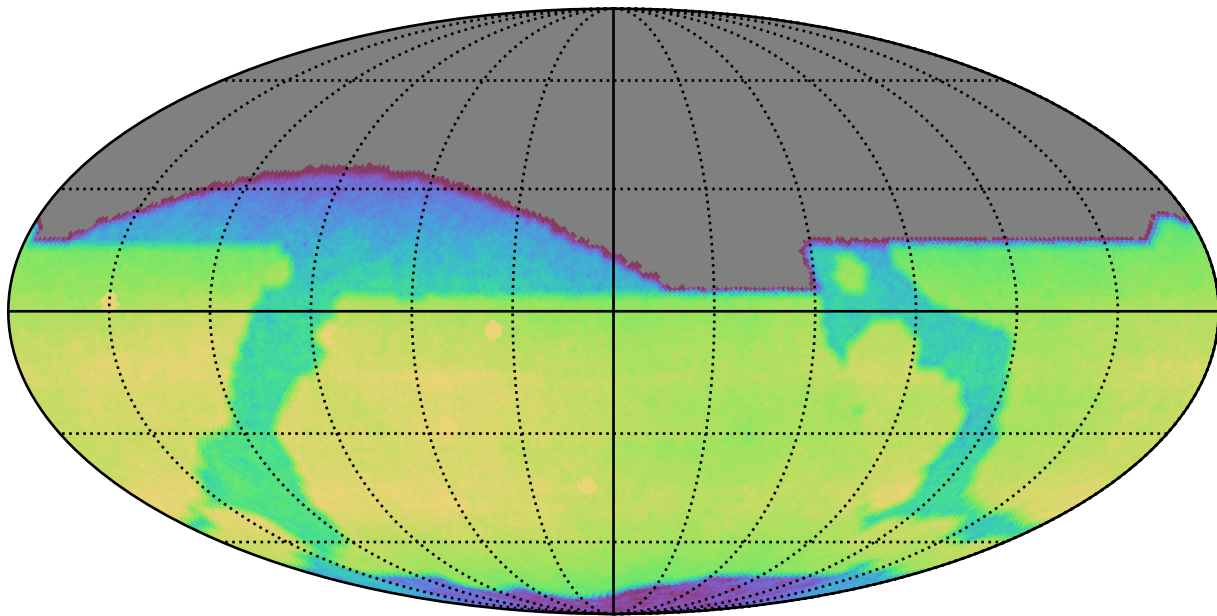
too_elab_r8_d3_griz_v3.4_10yrs All sky r band: CoaddM5
