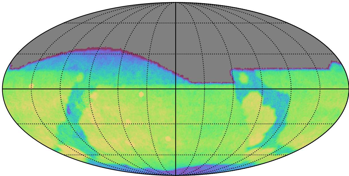
too_elab_r8_d3_griz_v3.4_10yrs All sky g band: CoaddM5
