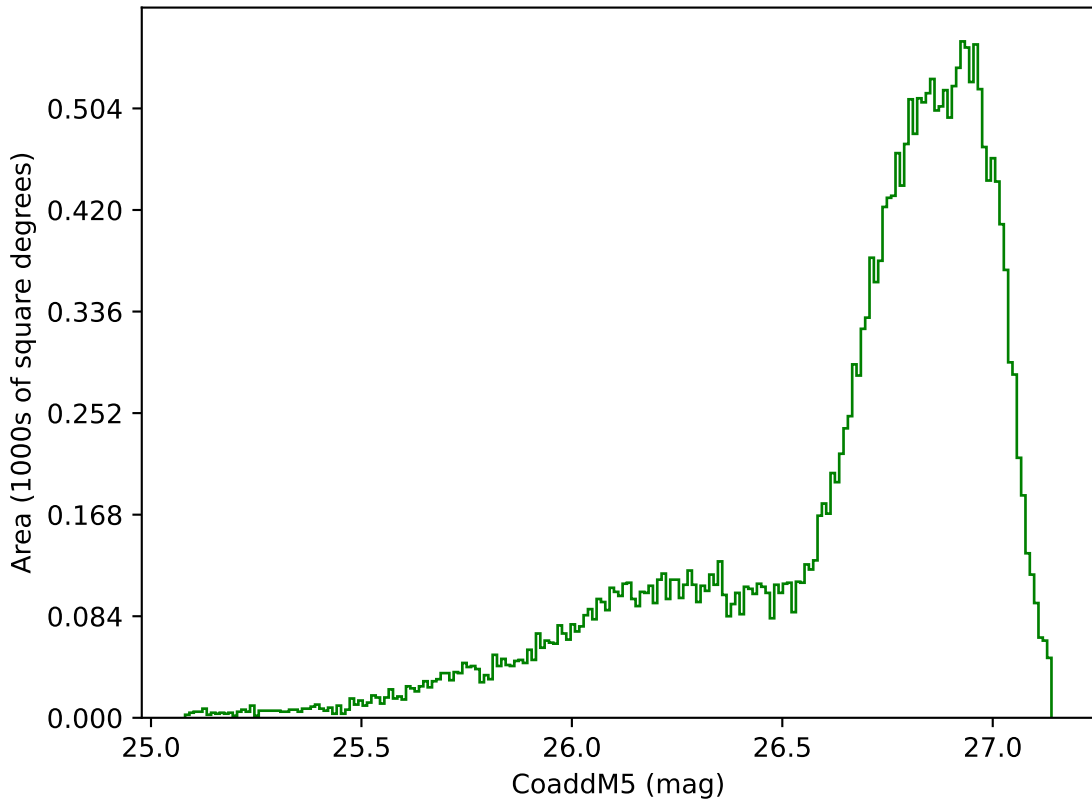
too_elab_r8_d3_griz_v3.4_10yrs All sky g band: CoaddM5
