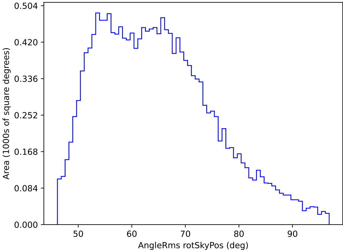
too_elab_r8_d3_griz_v3.4_10yrs WFD u band: AngleRms rotSkyPos
