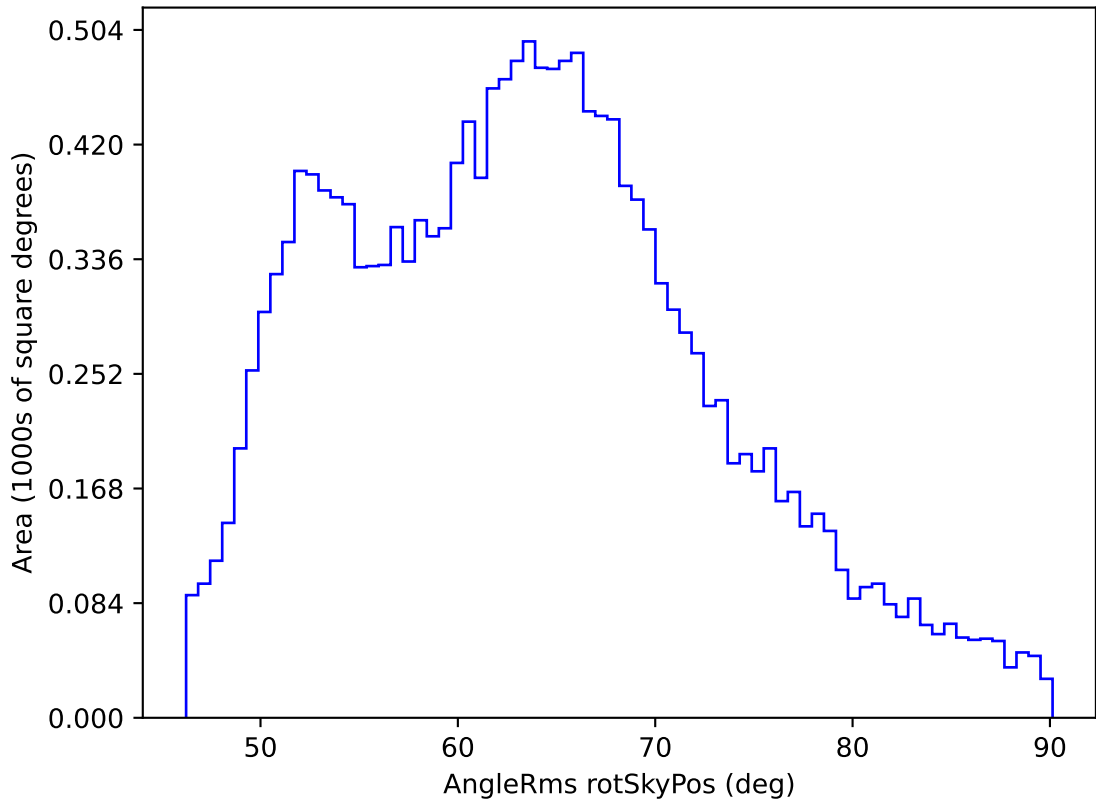
too_elab_r8_d3_griz_v3.4_10yrs WFD i band: AngleRms rotSkyPos
