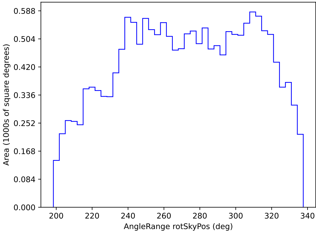
too_elab_r8_d3_griz_v3.4_10yrs WFD y band: AngleRange rotSkyPos
